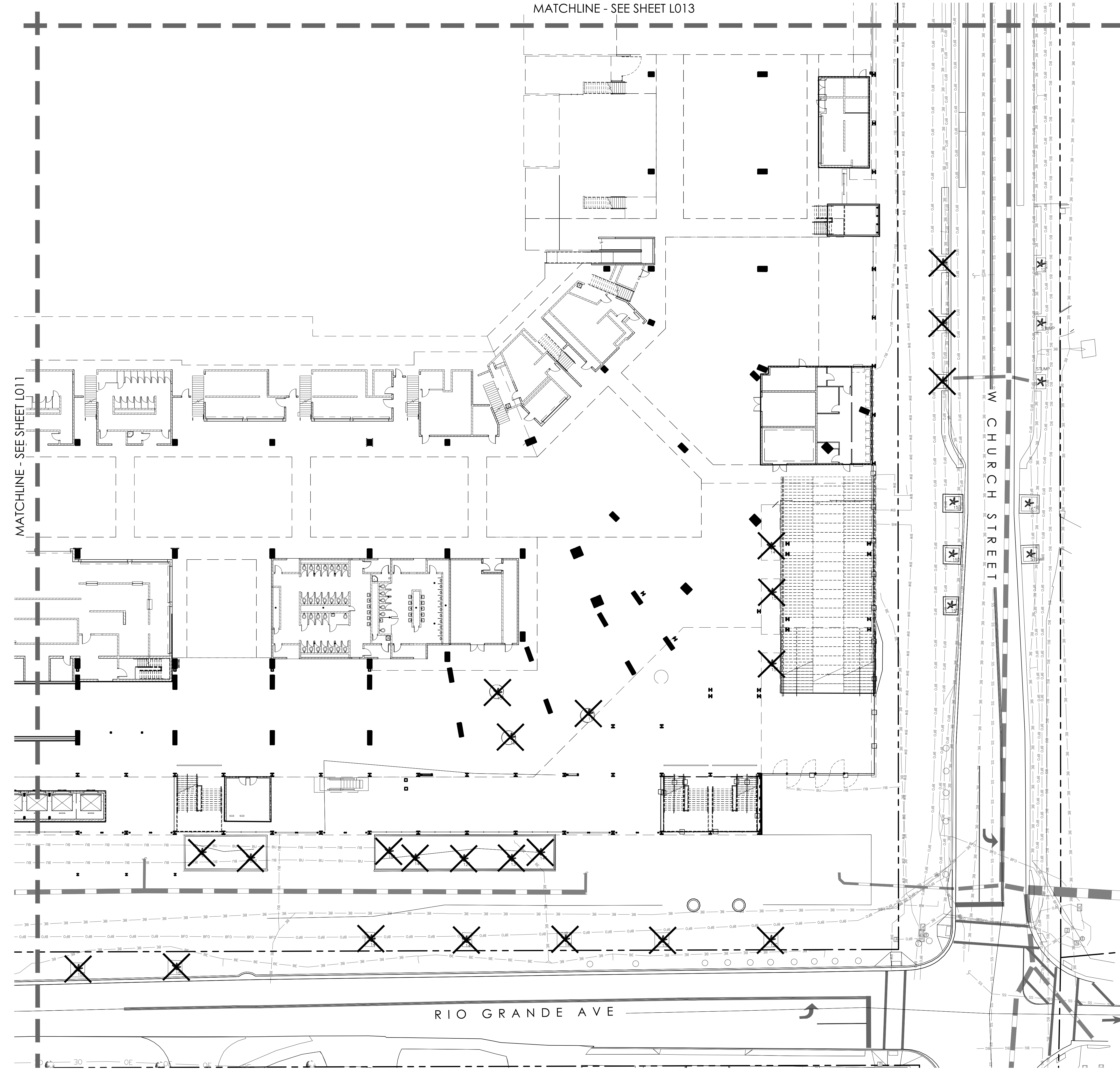
1 AREA B - LANDSCAPE REMOVAL CONCEPT PLAN SCALE: 1" = 20'
