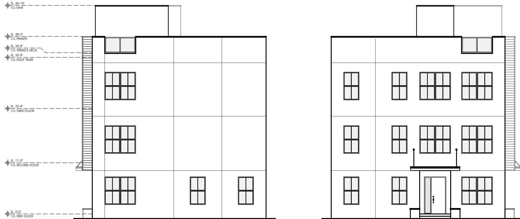
BUILDING I SIDE ELEVATIONS
