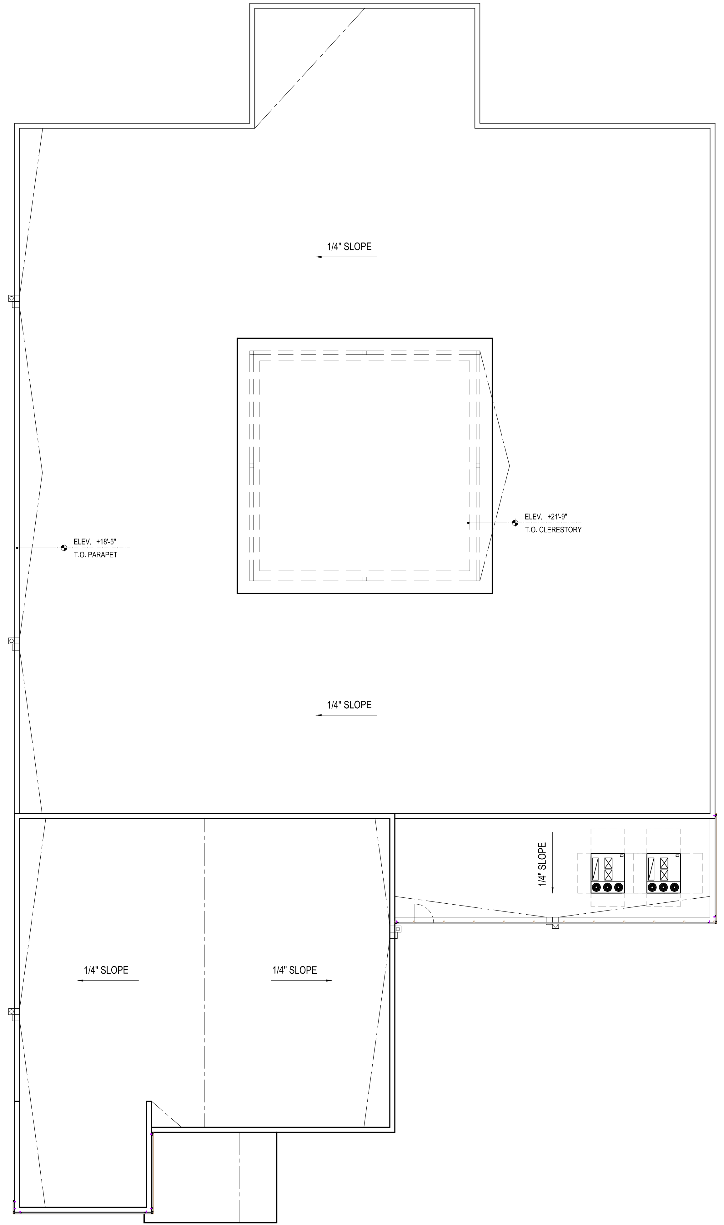
ROOF PLAN
