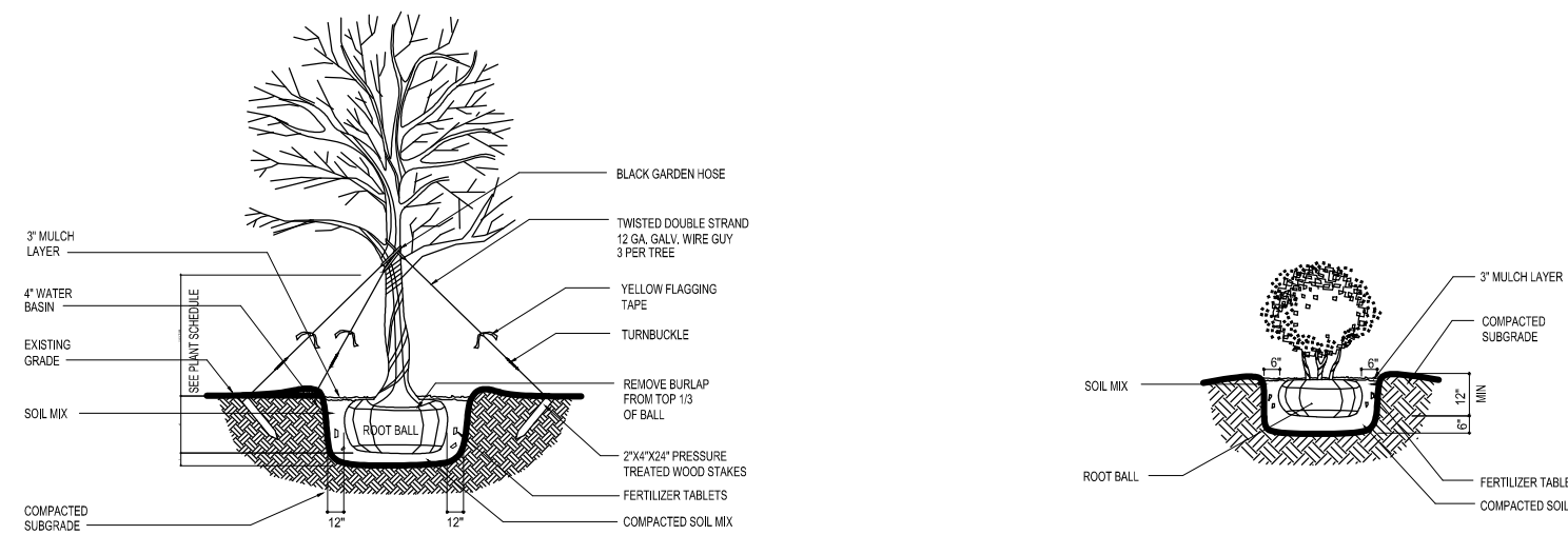
CANOPY TREE PLANTING DETAIL NOT TO SCALE
